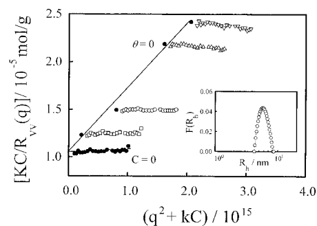
Figure 4. Typical Zimm plot of poly( N -2-ferrocenylethyl methacrylamide) in THF at 25 °C, where the concentrations are 4.30 \times 10^{-4} (squares), 1.61 \times 10^{-3} (hollow circles), 3.23 \times 10^{-3} (triangles), and 4.12 \times 10^{-3} g/mL (inverted triangles) and k = 5 \times 10^{17} mL/g. The inset shows a corresponding hydrodynamic radius distribution F(R_h) .
