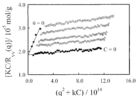
Figure 1. Typical Zimm plot of PFEMA-3 in toluene at 25 °C, where the concentrations are 3.92 \times 10^{-3} (hollow circles), 2.45 \times 10^{-3} (diamonds), 1.76 \times 10^{-3} (triangles), and 1.22 \times 10^{-3} g/mL (inverted triangles) and k = 5 \times 10^{16} mL/g.
