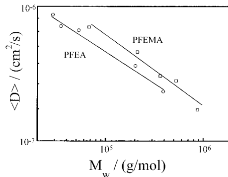
Figure 3. Double-logarithmic plots of \langle D \rangle vs M_w for PFEA and PFEMA in toluene at 25 °C, where the lines respond the least-squares fitting of \langle D \rangle = k_D M_w^{-\alpha_D} .
