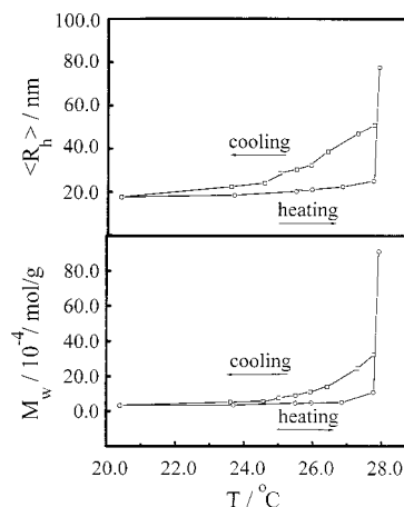
Figure 6. Temperature dependence of average hydrodynamic radius ( \langle R_h \rangle ) and weight-average molar mass M_w of poly(FEAA- co -NIPAM) with [FEAA]/[NIPAM] = 2:200 in water, where the concentration was kept at 7.6 \times 10^{-4} g/mL.
