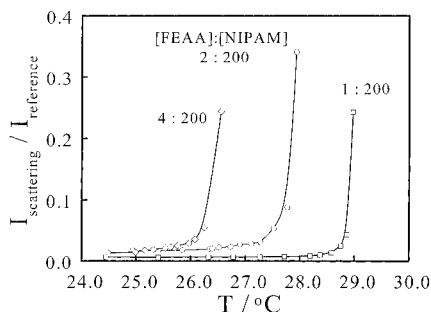
Figure 5. Temperature dependence of relative scattered light intensity ( I_{\text{scattering}}/I_{\text{reference}} ) in water for poly(FEAA- co -NIPAM), where the scattering angle is 60°.
